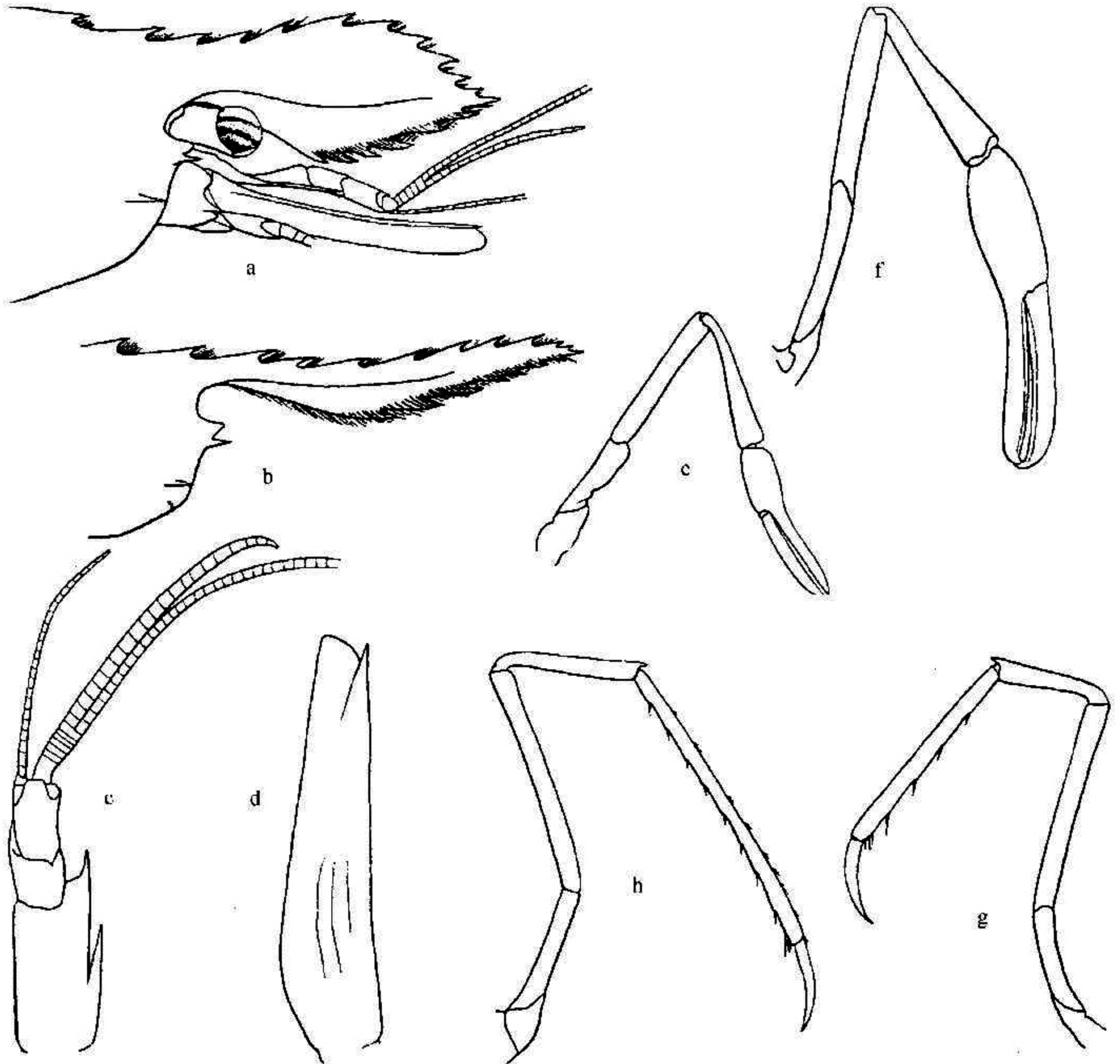
图 21 细角瘦虾 Leander tenuicornis (Say)
